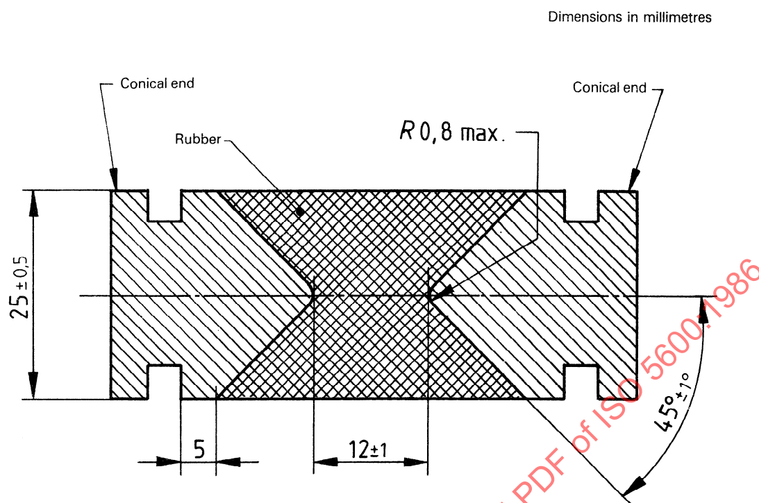
Figure — Standard test piece
