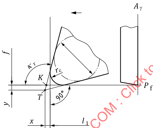
Figure 5 — Cutting edge angle \kappa_r > 90^\circ , with transverse feed for side cutting
