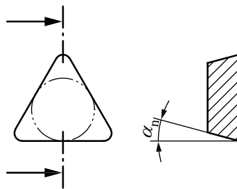
Figure 1 — Normal clearance \alpha_n
