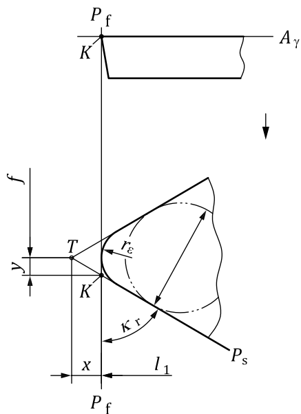
Figure 3 — Cutting edge angle \kappa_r \leq 90^\circ , with transverse feed for side cutting
