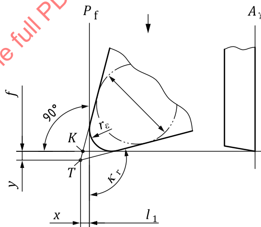
Figure 6 — Cutting edge angle \kappa_r > 90^\circ , with longitudinal feed for end cutting
