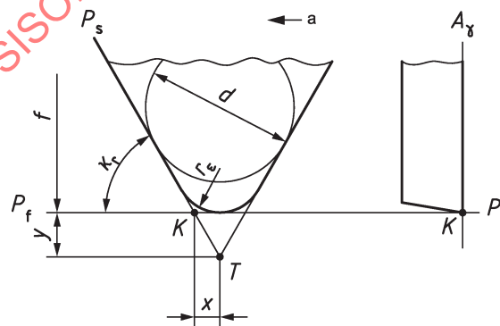
Figure 2 — Cutting edge angle \kappa_r \leq 90^\circ , with transverse feed
