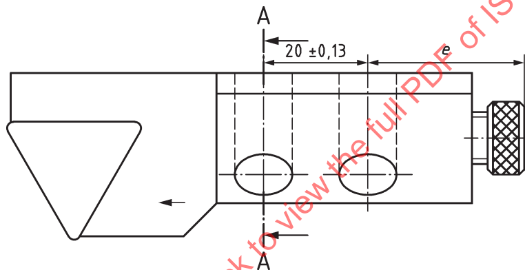
Figure 2 — Style W with height h_1 = 8 \text{ mm}, 10 \text{ mm}, 12 \text{ mm}, 16 \text{ mm} and 20 \text{ mm} with triangular indexable insert
