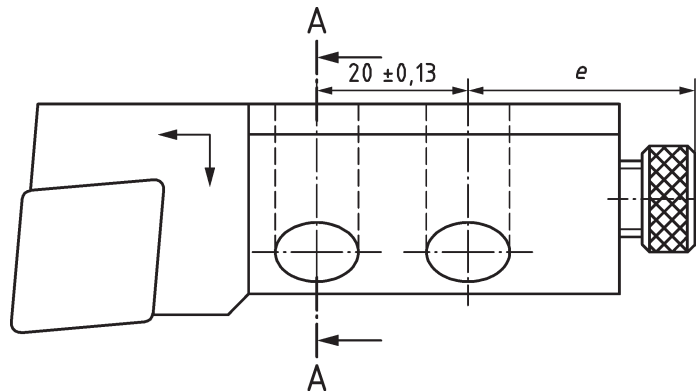
Figure 2 — Style L with height h_1 = 25 mm with rhombic indexable insert
