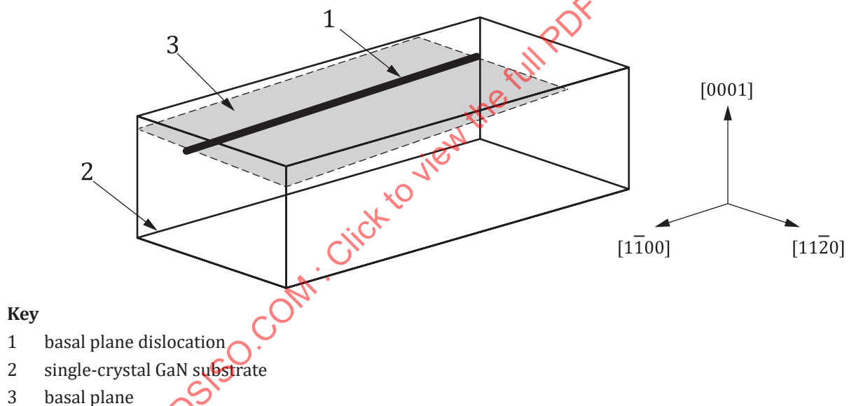
Figure 2 — Schematic illustration of a basal plane dislocation
