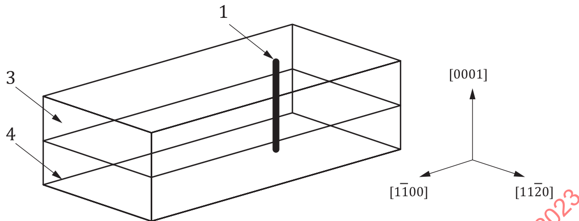
b) Schematic illustration of a threading dislocation in a GaN single-crystal film
