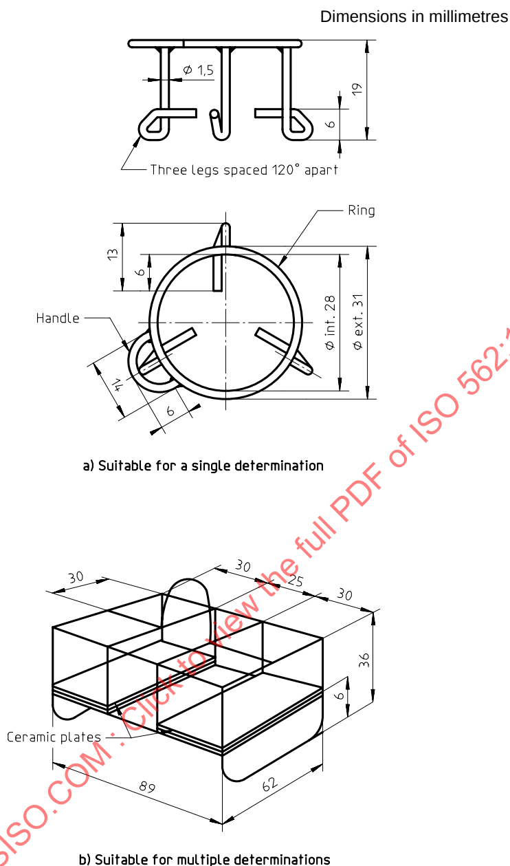
Figure 3 — Crucible stands
