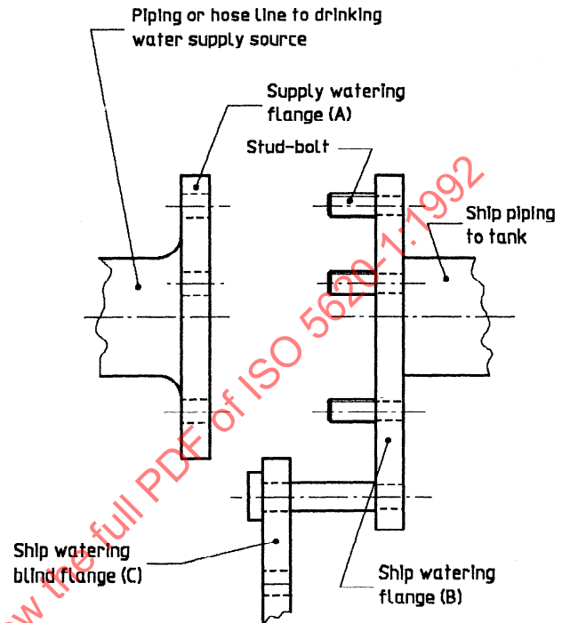
Figure 1 — Connection principle
