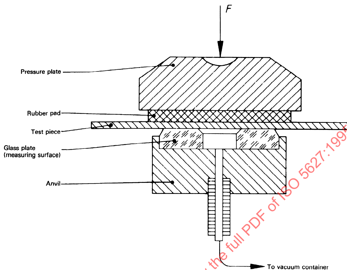
Figure 1 — Measuring principle
