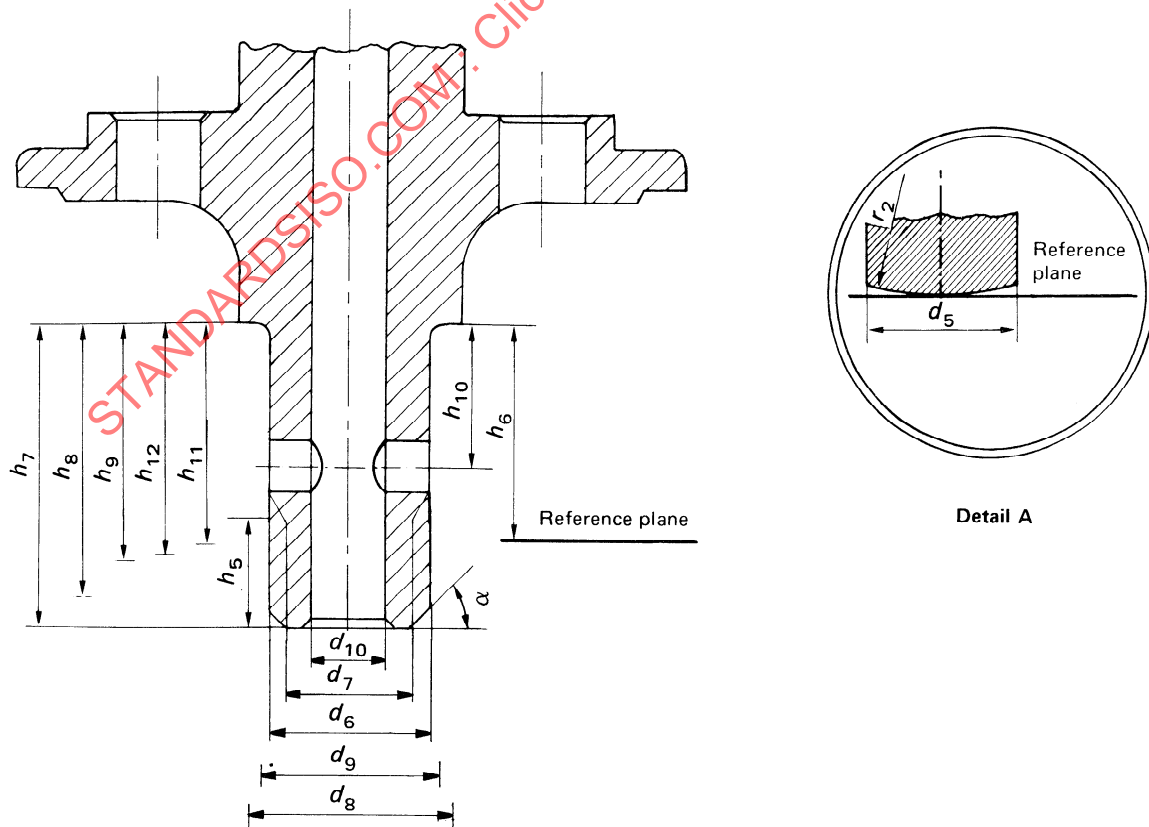
Figure 10 — Part detail of spindle lock
