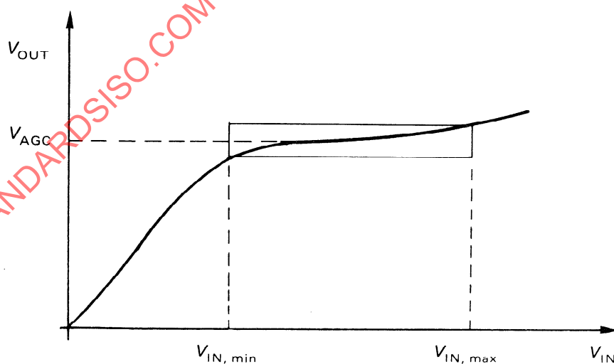
Figure 14 — AGC-amplifier characteristics
