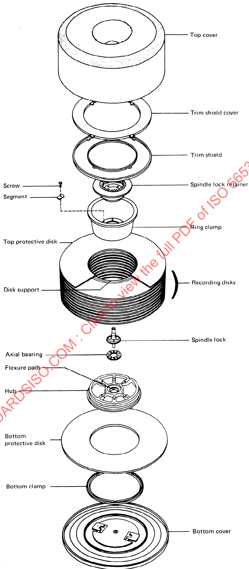
Figure 6 — Disk pack, exploded view
