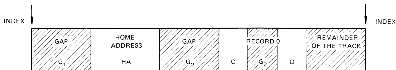
Figure 1 — Track layout of an initialized data track
