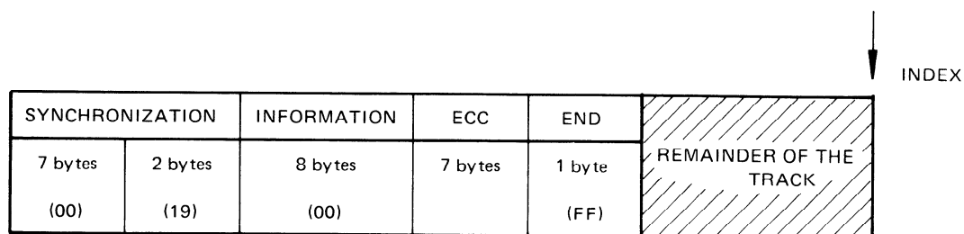
Figure 4 — Data block of record 0
