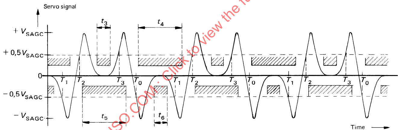
Figure 23 — Timing, amplitude and noise constraints for servo signal
