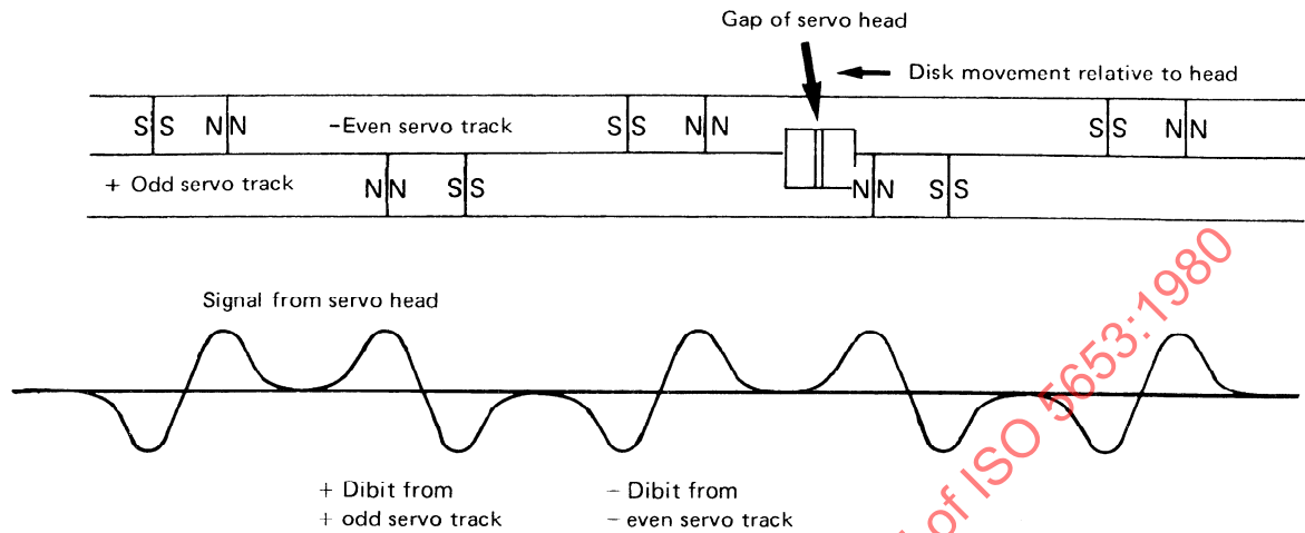
Figure 19 — Servo head signal at servo tracking centreline
