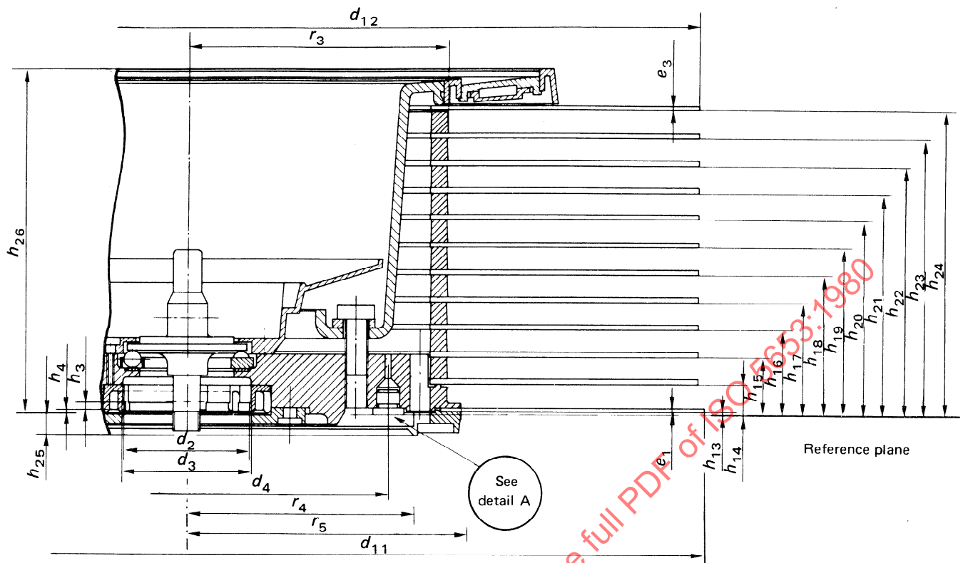
Figure 9 — Partial cross-section of disk pack
