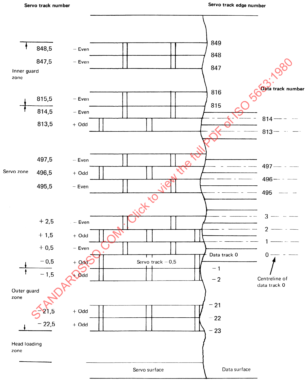
Figure 21 — Relationship between tracks on servo and data surfaces
