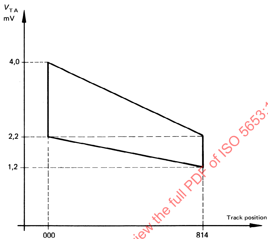
Figure 15 — Track average amplitude
