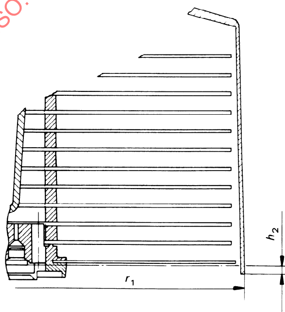
Figure 8 — Top cover/ pack centreline relationship
