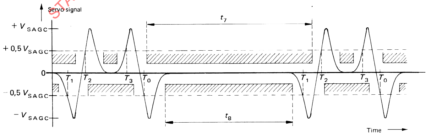
Figure 24 — Noise constraints for index pattern
