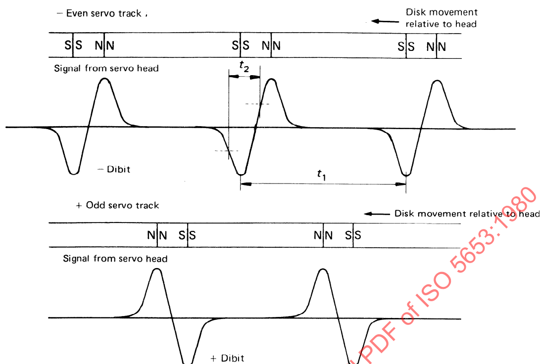
Figure 17 — Minus-even and plus-odd tracks
