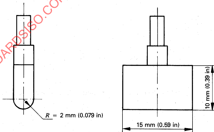
Figure 13 — Stylus
