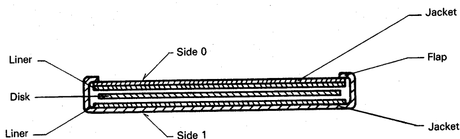
Figure 2 — Section A-A
