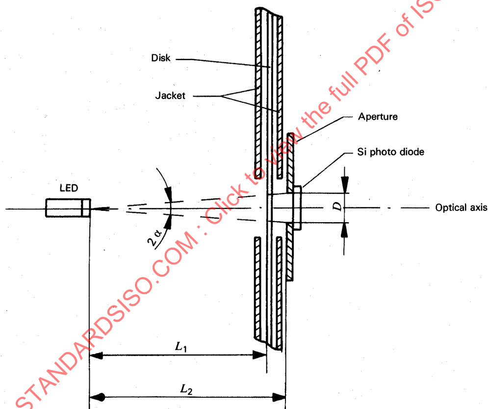
Figure 9 — Measuring device
