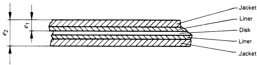
Figure 5 — Cartridge jacket thickness
