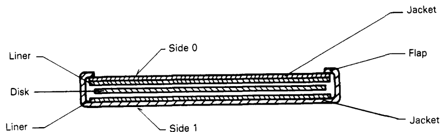
Figure 2 — Section A-A
