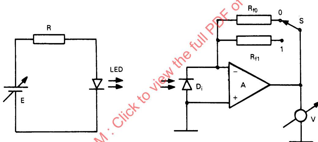
Figure 10 — Electronic circuitry
