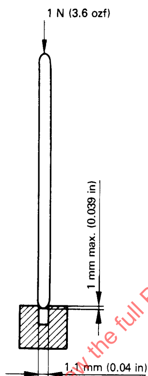
Figure 12 — Measuring gauge
