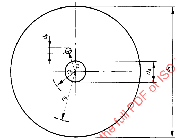
Figure 6 — Disk dimensions
