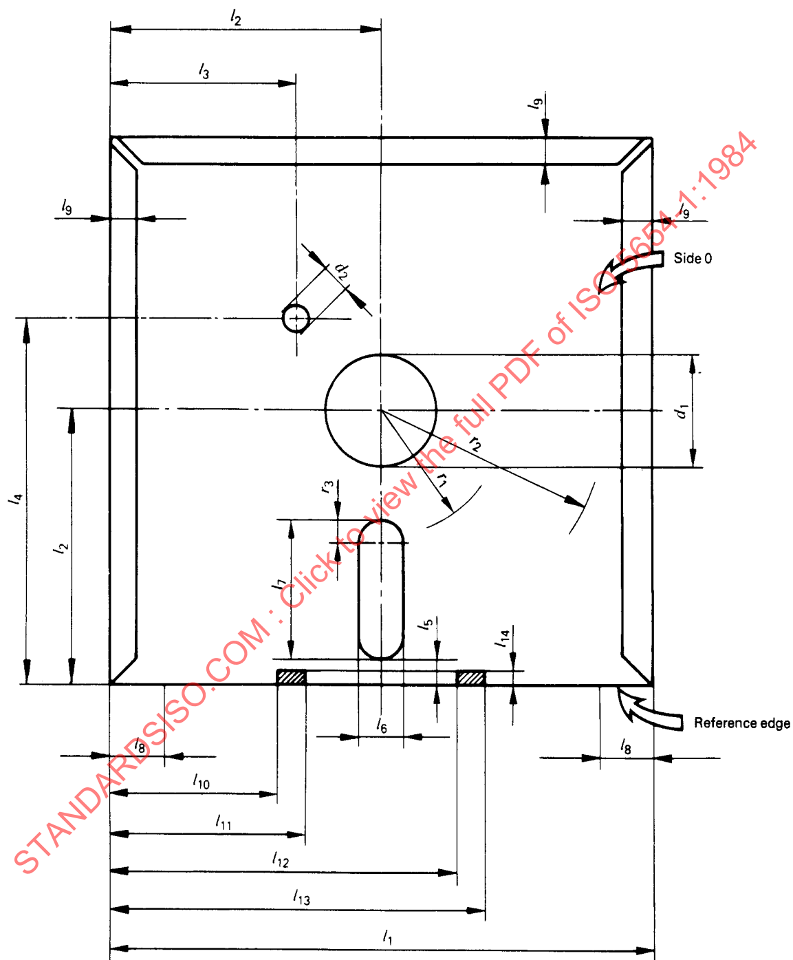
Figure 4 — Jacket dimensions
