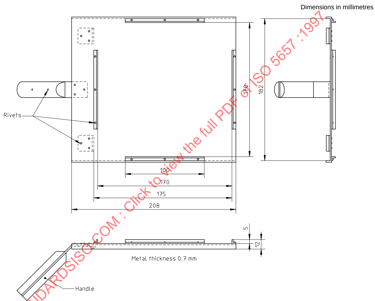
Figure 7 — Specimen insertion and location tray
