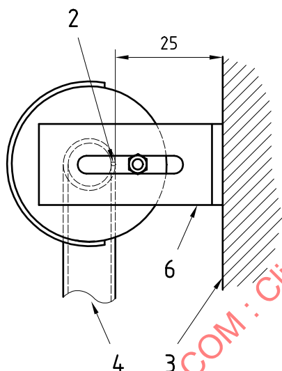
b) Burner position to specimen surface [side view on a)]
