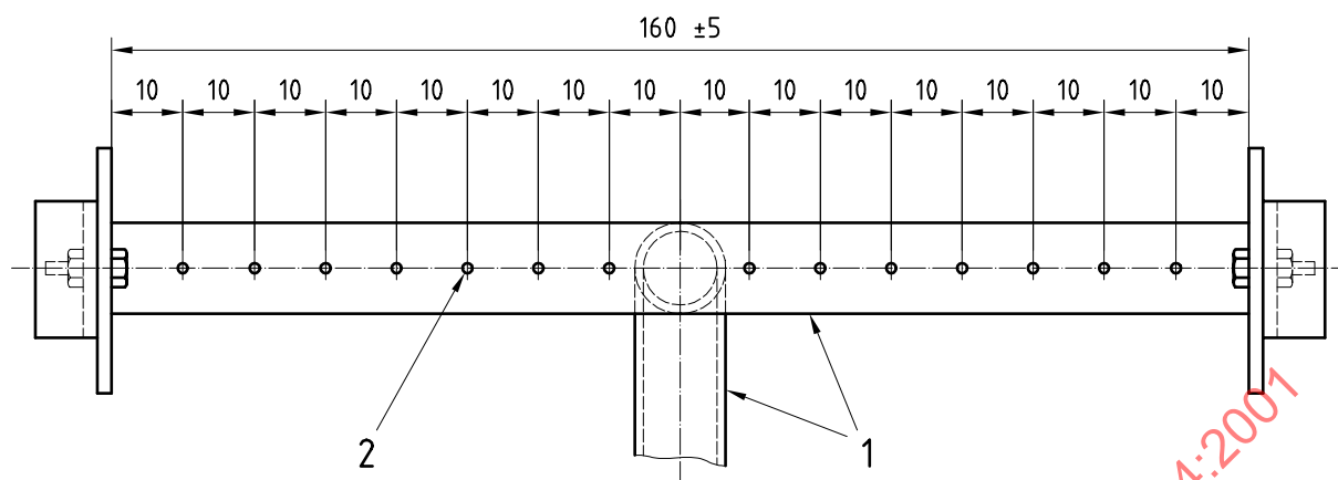
a) Hole separations on burner tube (front view with draught screen omitted)
