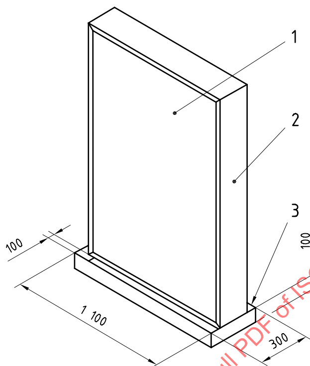
a) General arrangement
