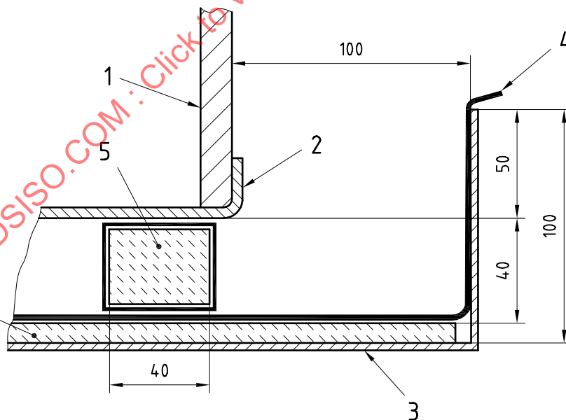
b) Position of debris collection tray and showing lining to tray
