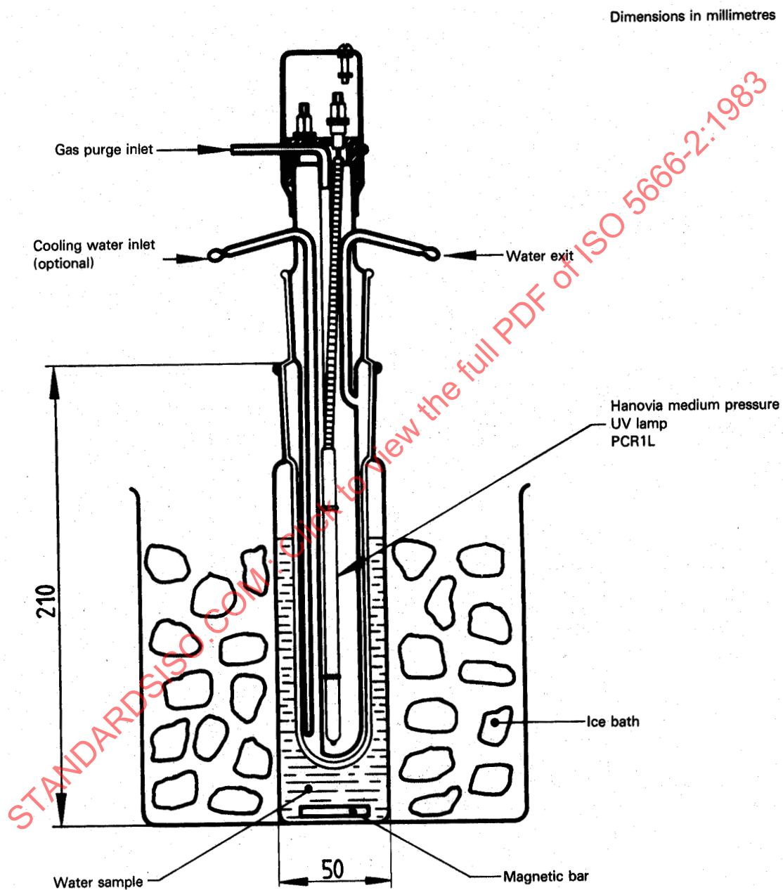
Figure 1 — Apparatus for UV irradiation (capacity 100 ml)
