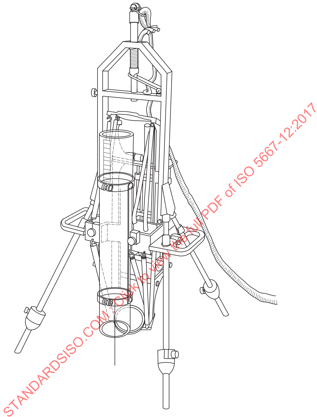
Figure H.1 — Jenkins mud sampler
