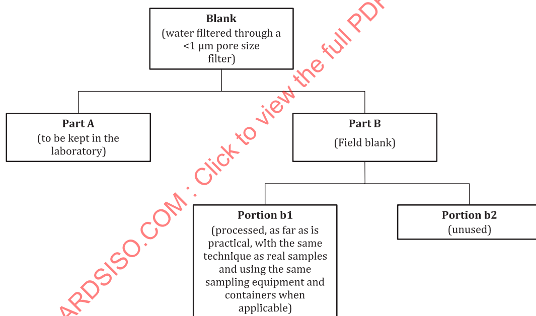
Figure 1 — Flow chart of the the field blank sampling technique for grab sampling
