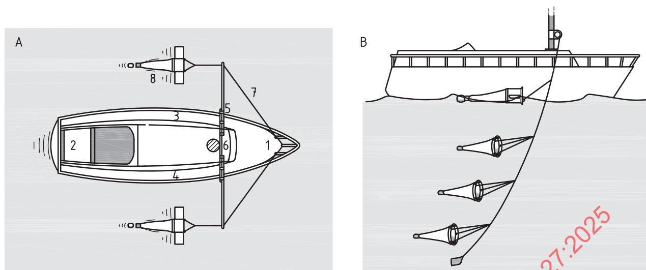
a) Schematic setup for dynamic sampling of surface waters using manta or neuston nets
