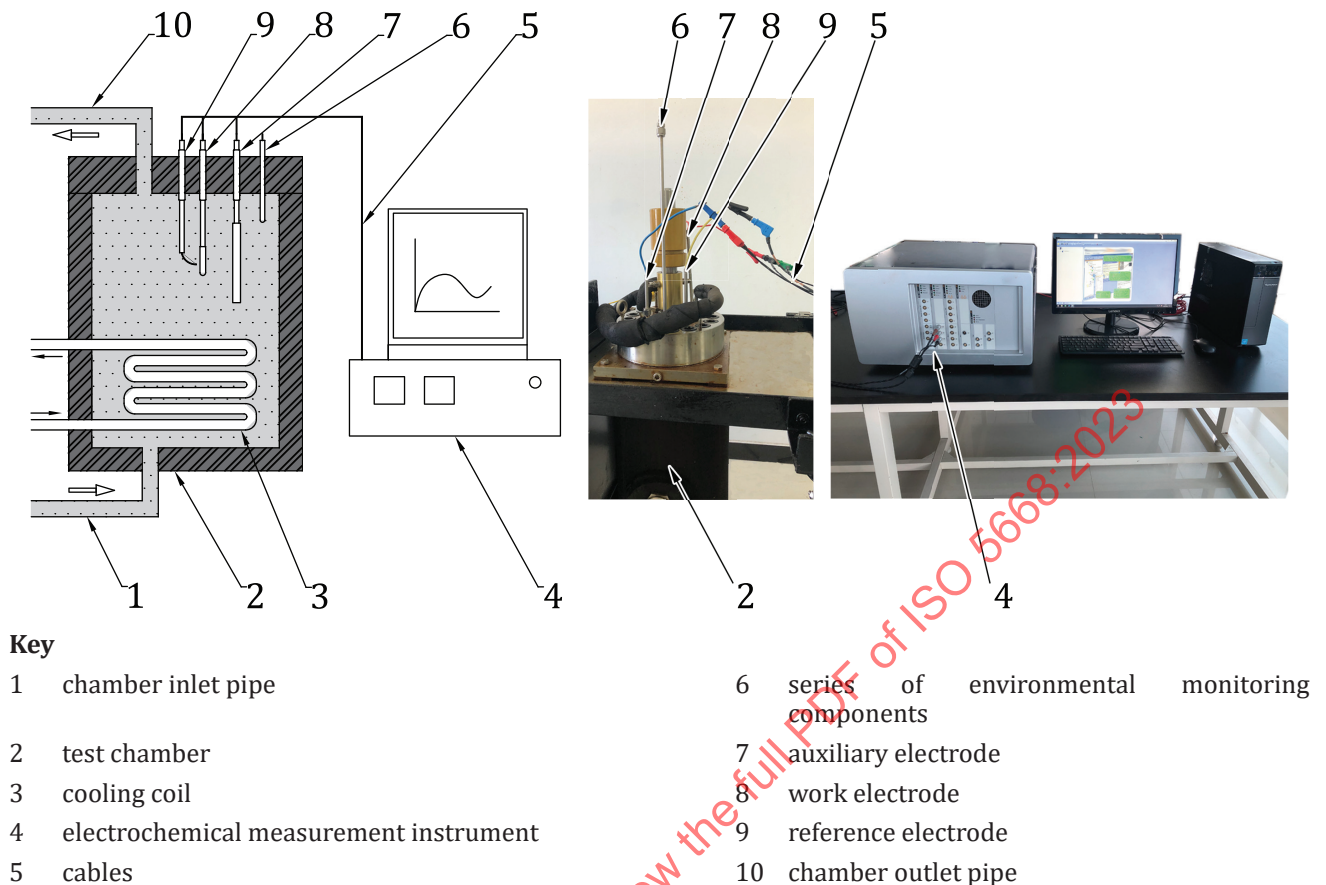
Figure 3 — Schematic diagram and actual setup of simulated deep-sea environment test chamber for electrochemical test
