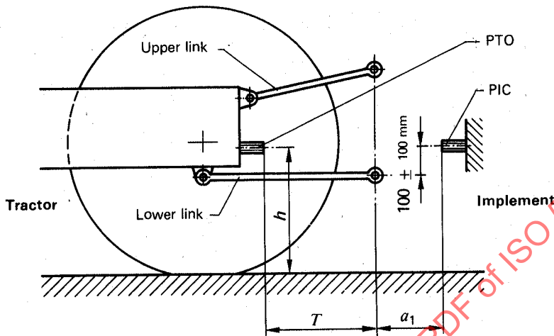
Figure 2 — Positioning of PIC for mounted implements
