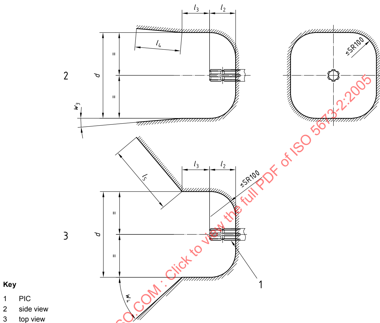
Figure 7 — Minimum PTO drive-line clearance envelope at PIC for three-point linkage attachment
