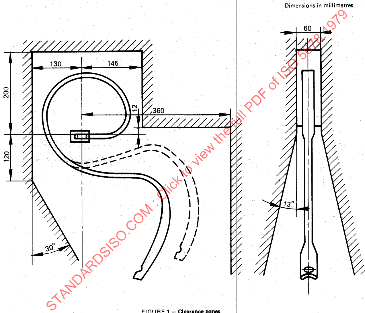
FIGURE 1 — Clearance zones
