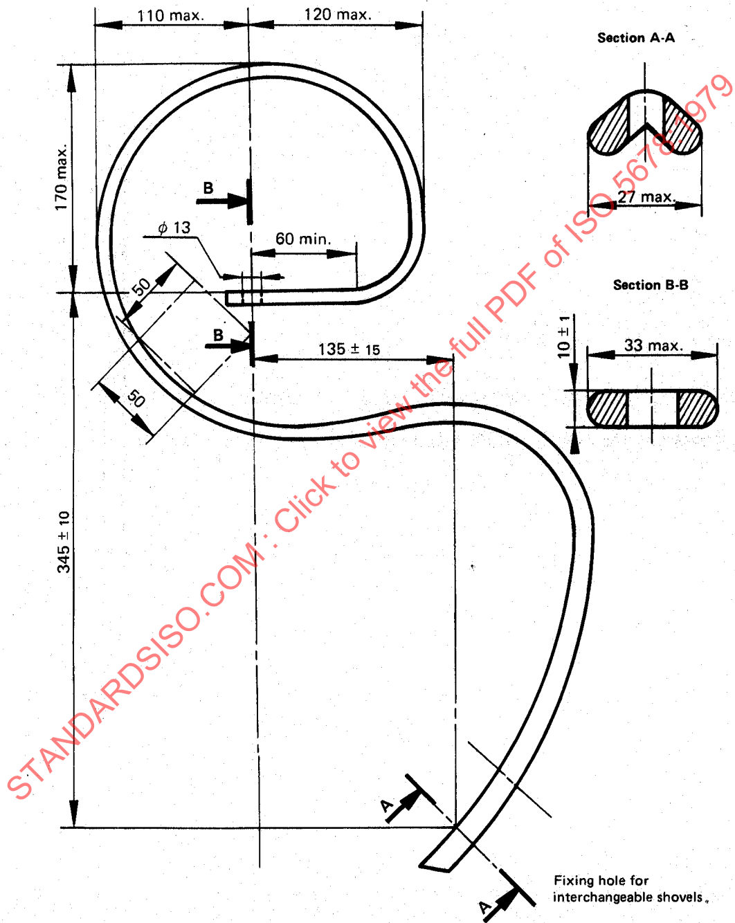
FIGURE 2 -- Main dimensions
