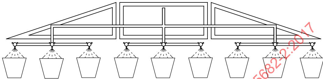
Figure 2 — Nozzle flow rate measurement test method
