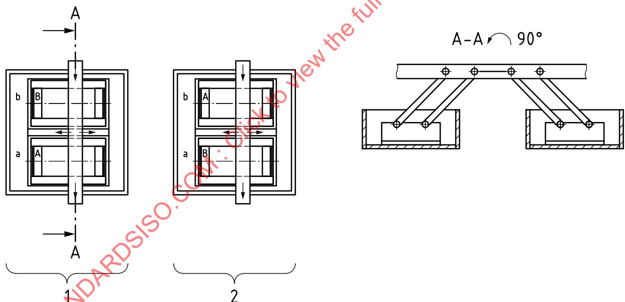
Figure 10 — Parallel positions of the specimen boxes with self-supporting arms extending from the centre
