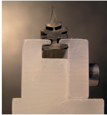
Figure 5 — Insertion of the wiper rubber
