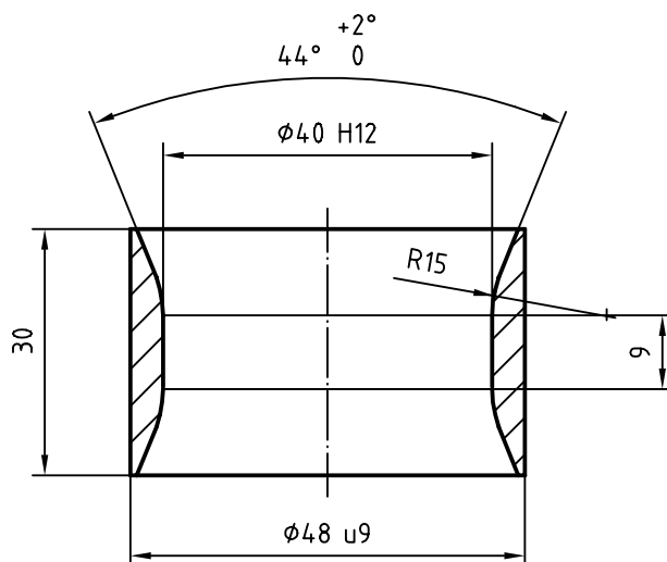
Figure 3 — Socket
