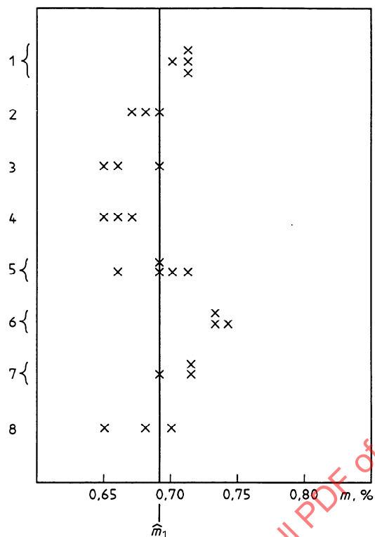
Figure B.1 — Sulfur content of coal, sample 1
