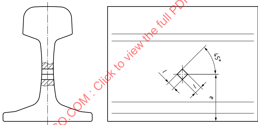
Figure C.3 — Simulated transverse fissure in web A
