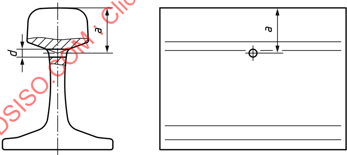
Figure B.11 — Bolt hole slot, position D
