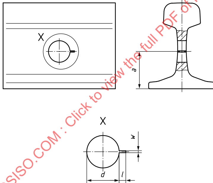
Figure B.6 — Transvers slot in rail head
