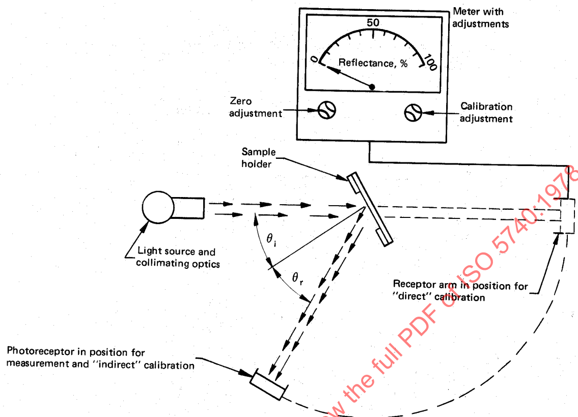
FIGURE 1 — Generalized reflectometer showing geometries for the two calibration methods
