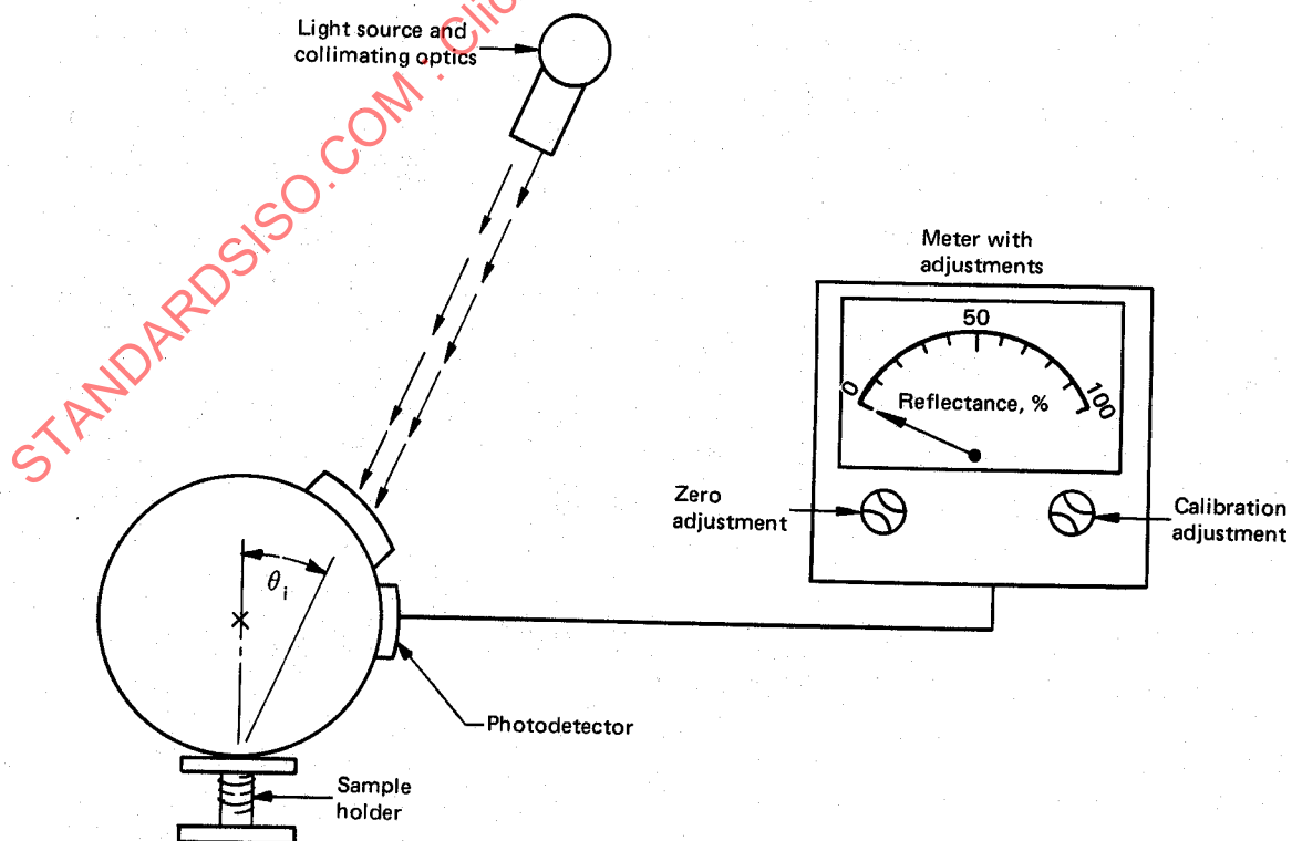
FIGURE 2 — Generalized reflectometer, incorporating an integrating sphere in the receiver
