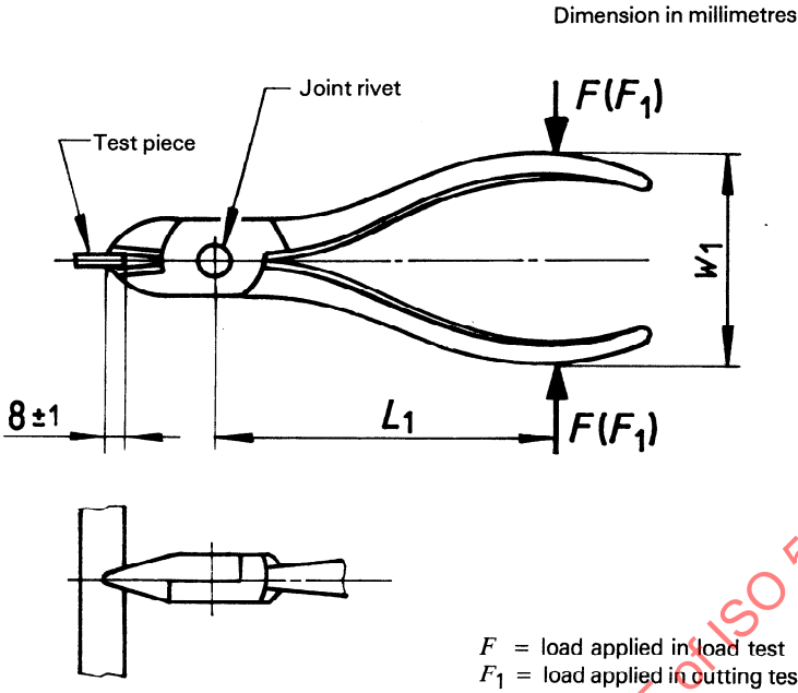
Figure 1 — Diagonal cutting nipper
