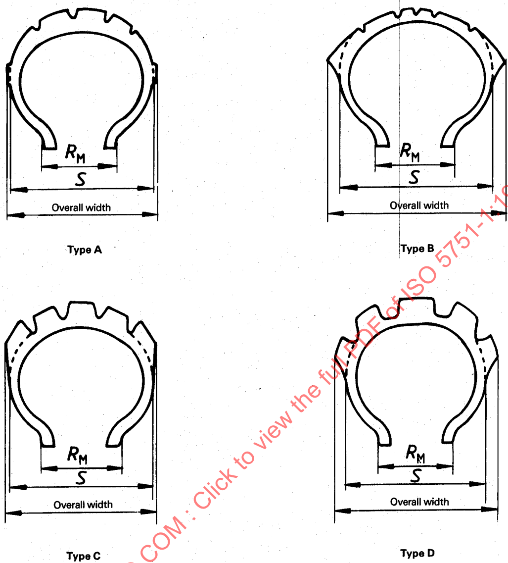
Figure — Tread configurations
