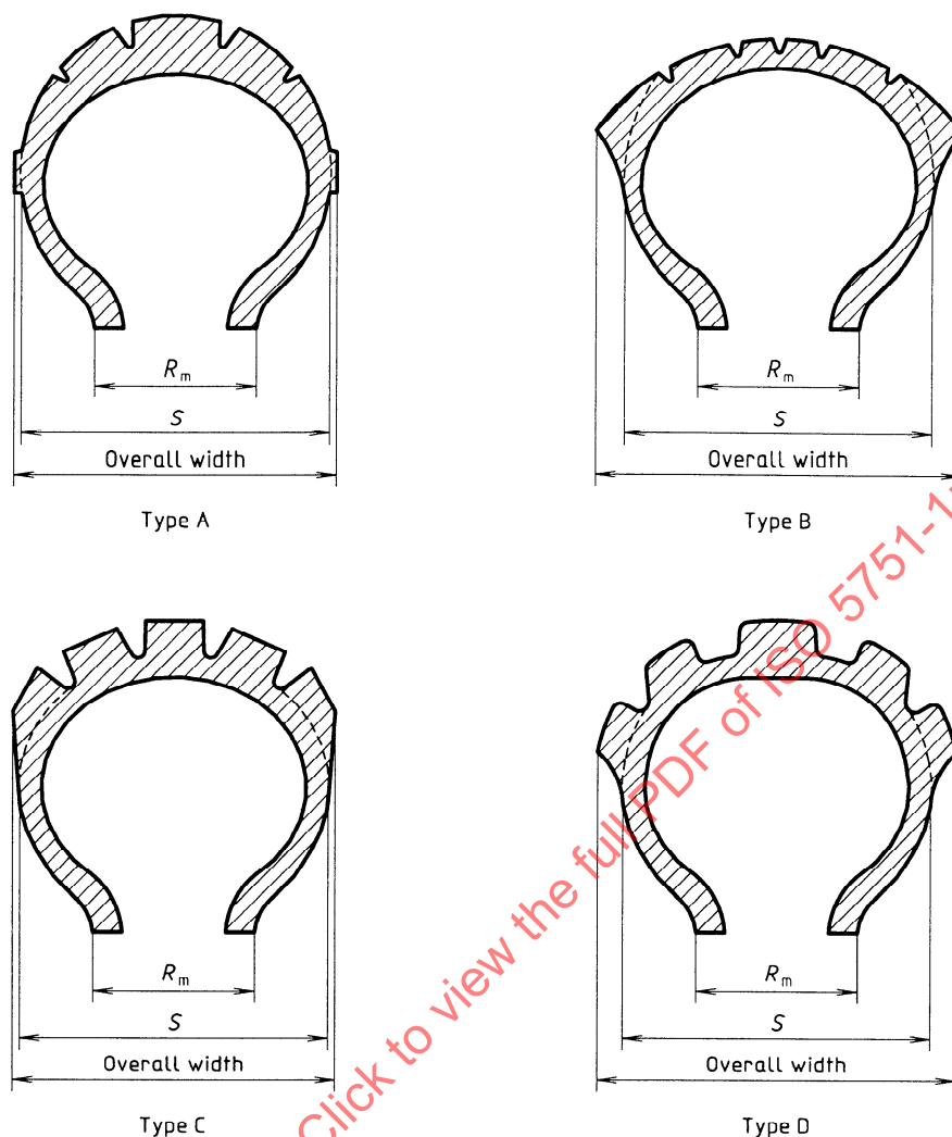
Figure 1 — Tread configurations
