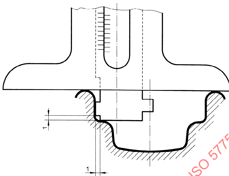
Figure A.7 — Vernier gauge with 1/20 mm graduations
