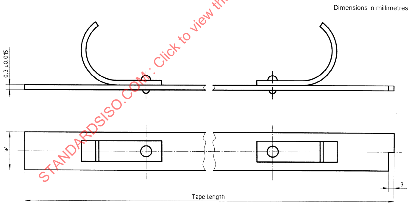
Figure A.5 — Tape dimensions
