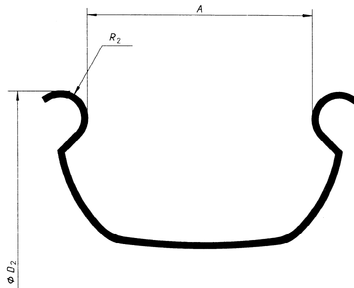
Figure A.2 — Hooked bead rims
