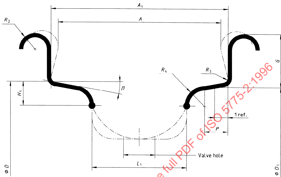
Figure 1 — Straight side rims
