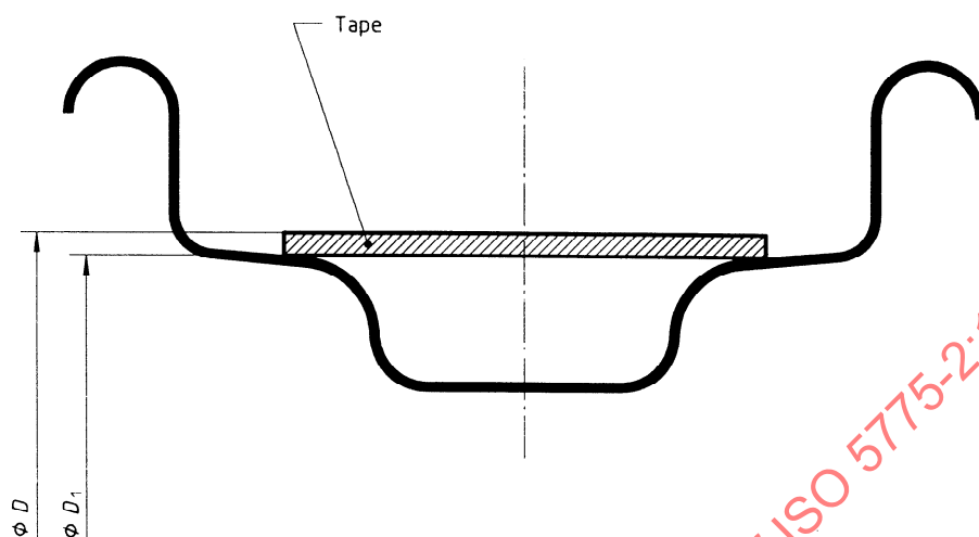
Figure A.4 — Rim diameter measurement
