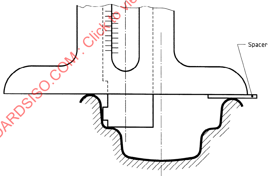
Figure A.8 — Use of vernier gauge with spacer
