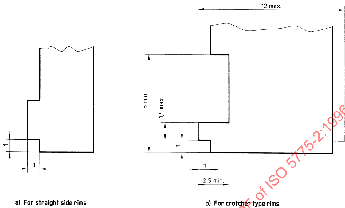
Figure A.9 — Vernier gauge details for measuring flange height G
