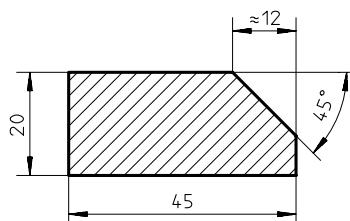
Figure 7 — Hatch seal, cross-section
