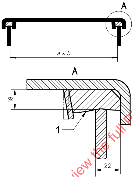
Key 1 Hatch seal
