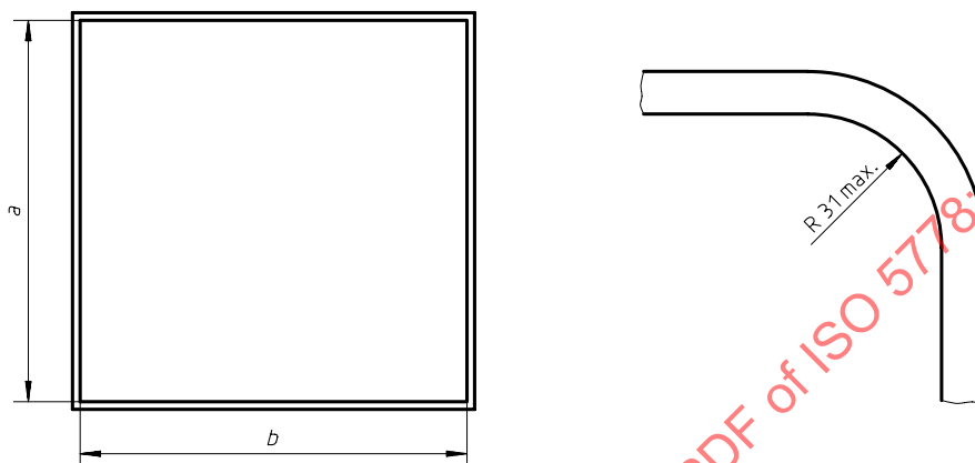
Figure 2 — Upper part of coaming
