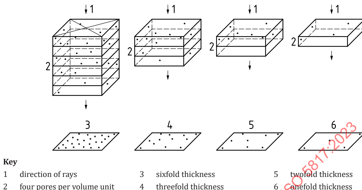
Figure 1 — Radiographic films of specimens with identical occurrence of pores per volume unit
