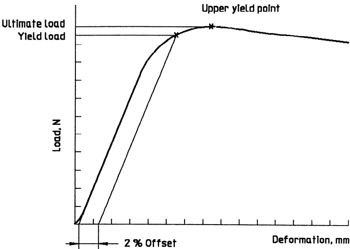
Figure E.2 — Idealized load/deformation curve for cement
