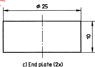
Figure E.1 — Mould for preparing compressive strength test specimens
