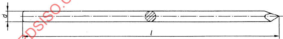
Figure 1 — Main dimensions of skeletal pins
