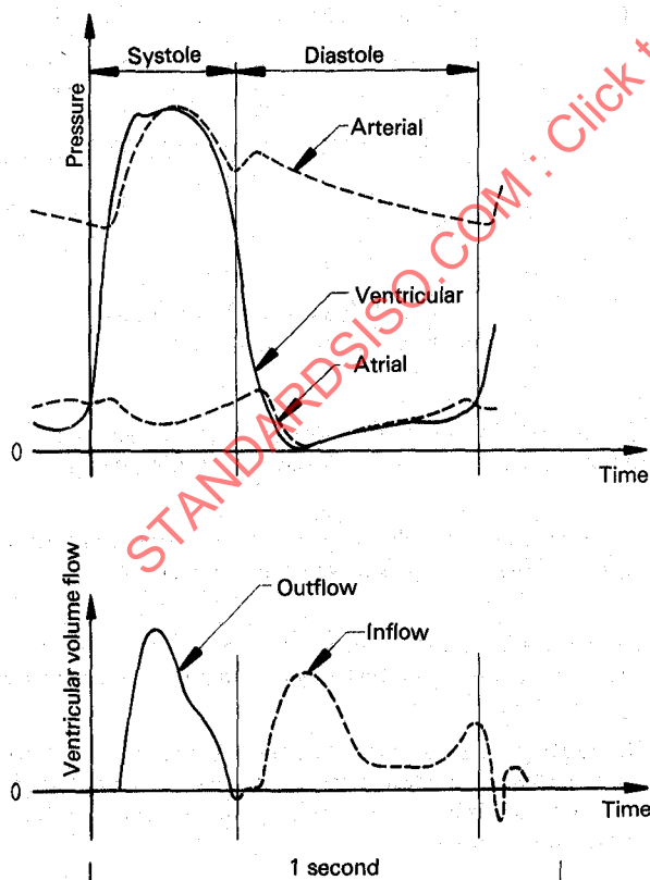
Figure 3 — Diagrams of haemodynamic wave-forms, simulating those of healthy humans
