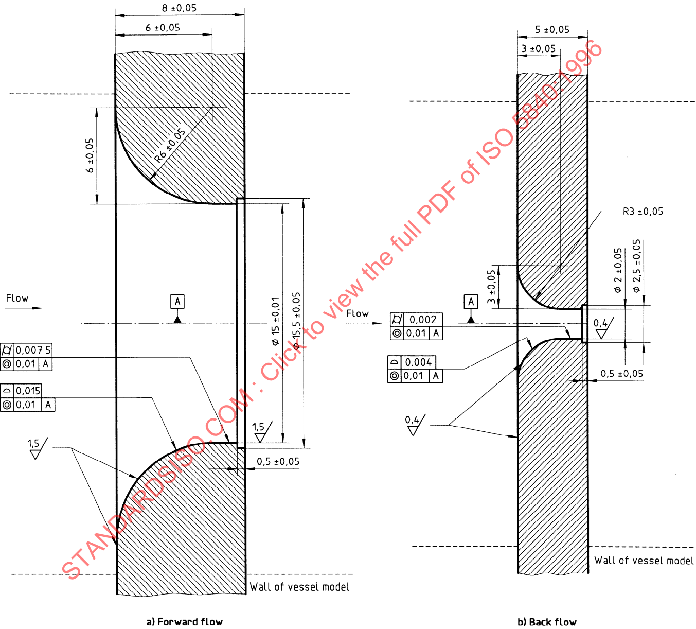
Figure 3 — Standard nozzle
