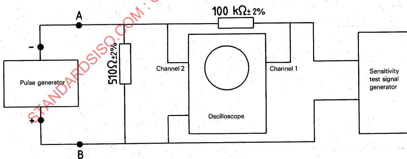
Figure 2 — Circuit diagram for sensitivity measurements
