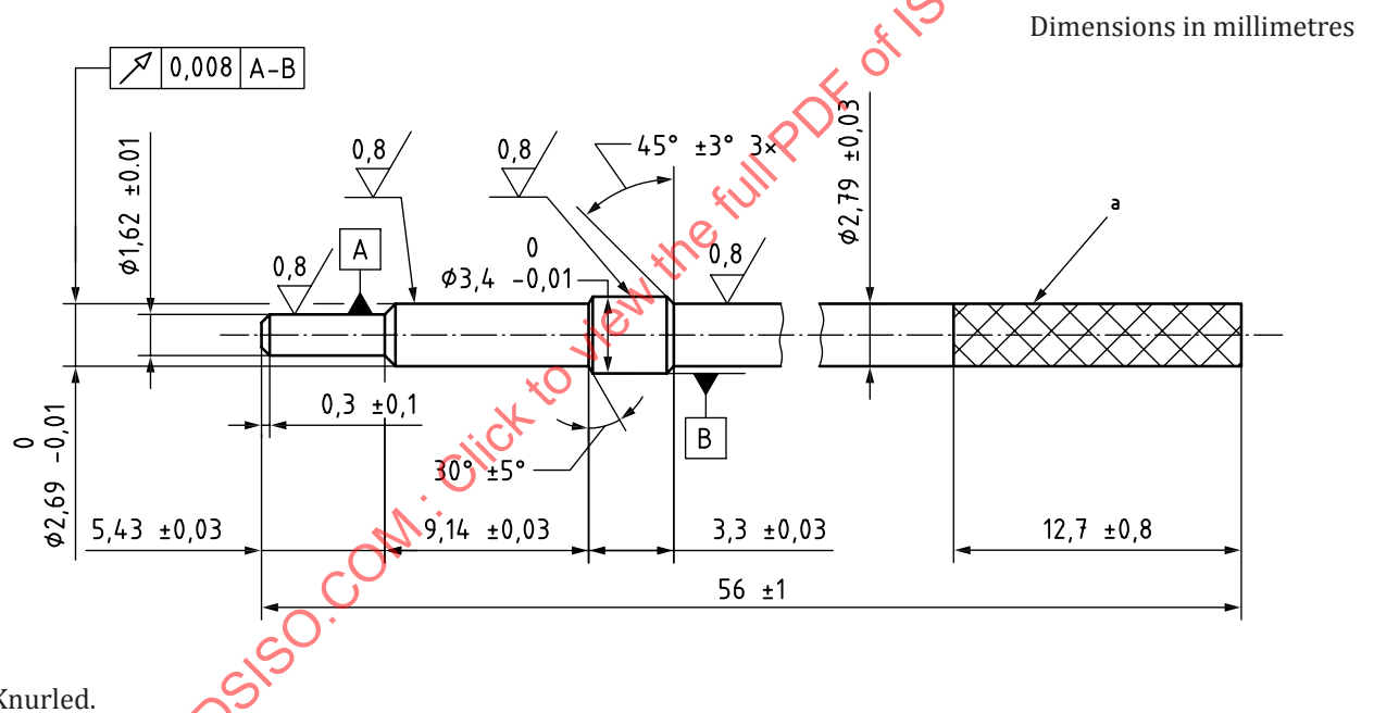
Figure 5 — Connector cavity GO gauge
