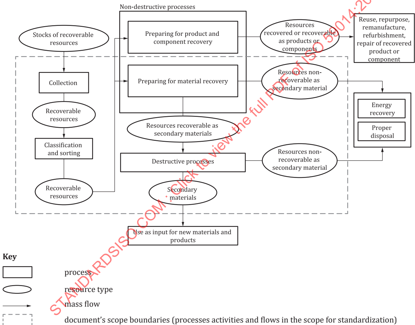
Figure 3 — Simplified representation of activities and processes for recovering secondary materials
