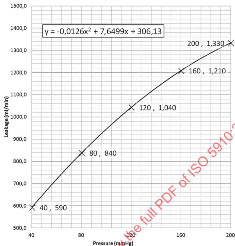
Figure M.2 — Back flow nozzle gradients
