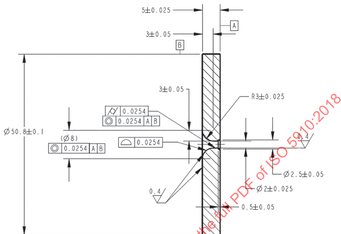
Figure M.1 — Standard nozzle; back flow (dimensions in millimetres)
