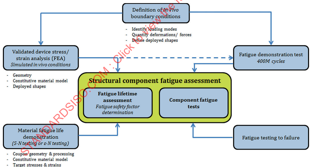
Figure O.1 — Example schematic of a structural component fatigue assessment using a stress or strain-life approach
