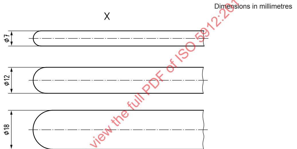
Figure 8 — Test probe
