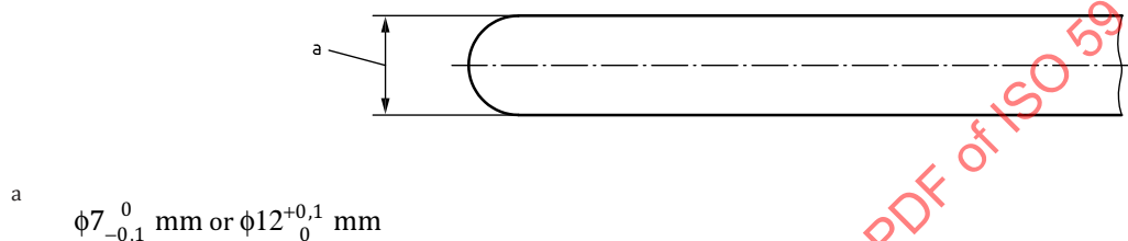
Figure 8 — Measuring probes
