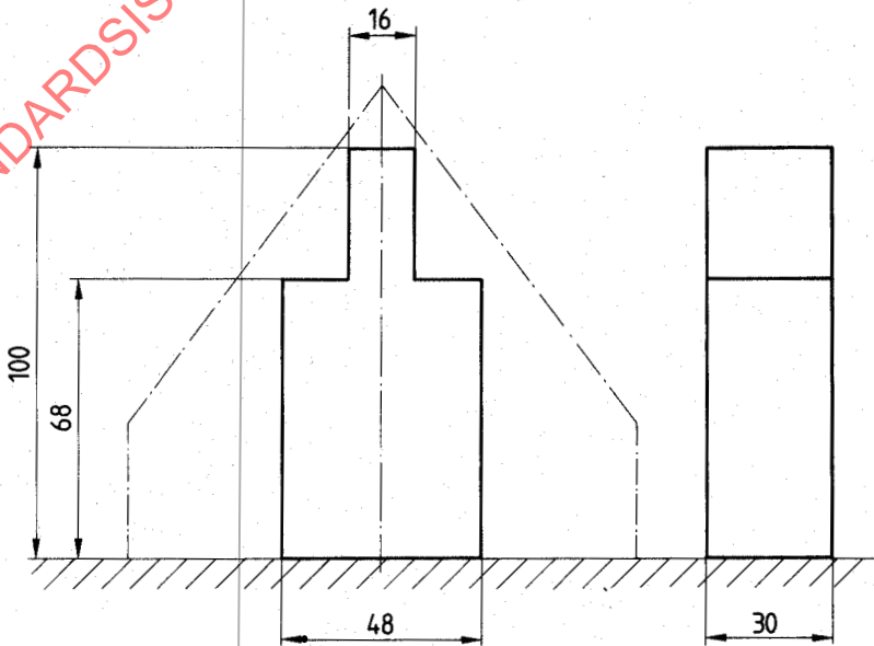
Figure 1 — Test body for clear height and seats
