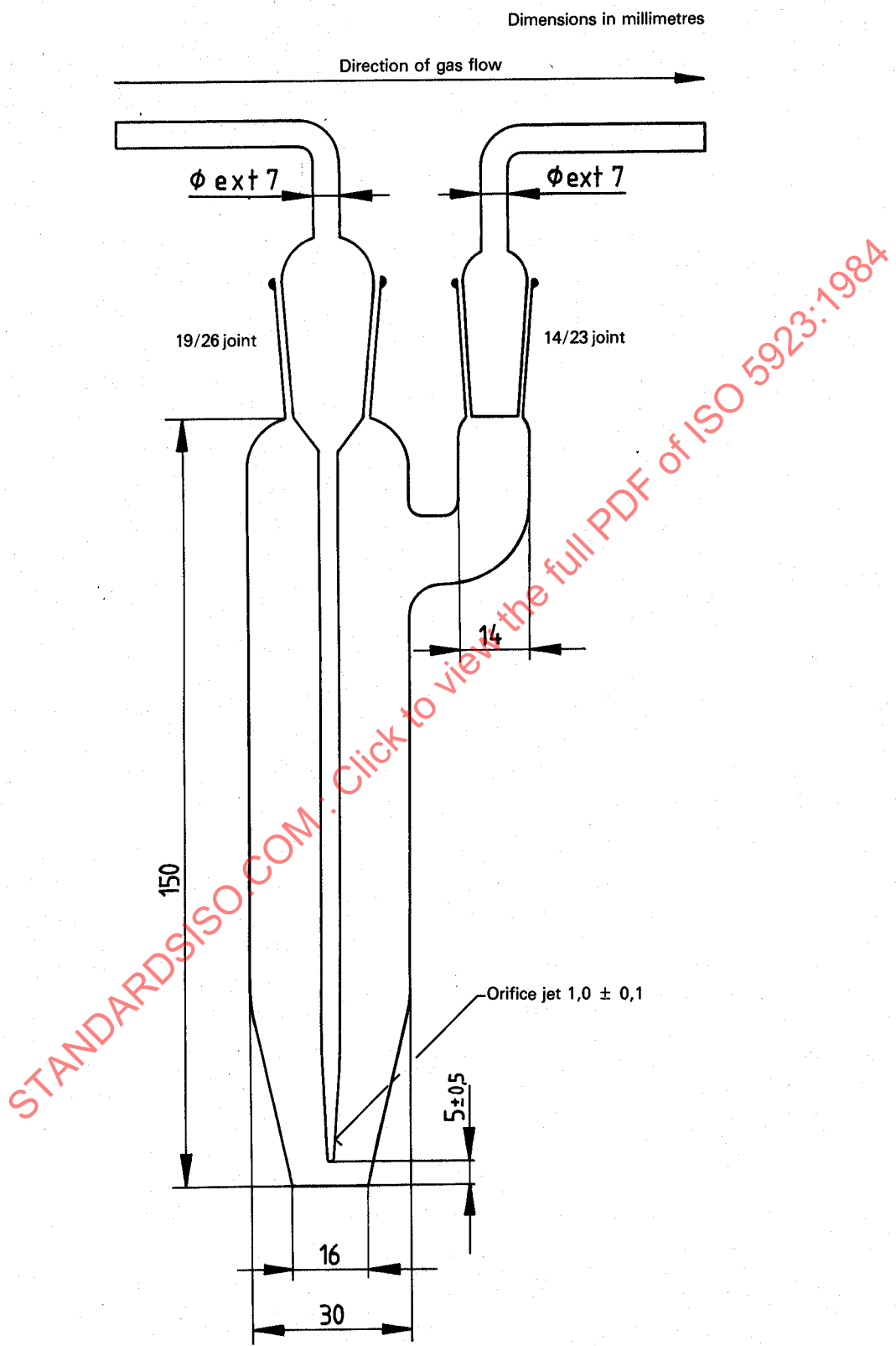
Figure 1 — Bubbler for the determination of oil content
