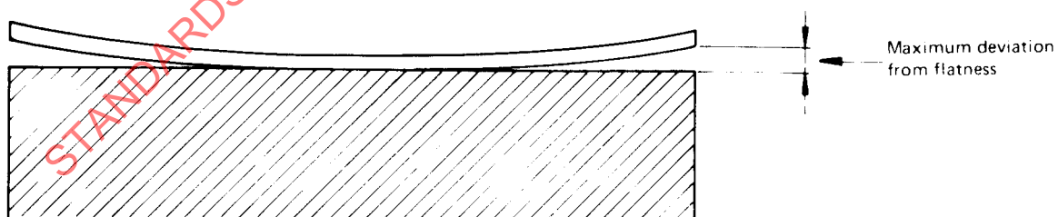
Figure 4 — Measurement of flatness
