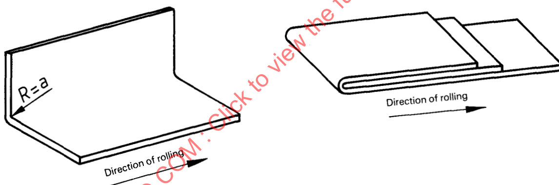
(a) 90° transverse bend around a radius of 1 a
