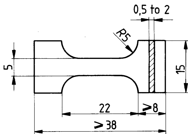
Figure 7 — PTFE Specimen
