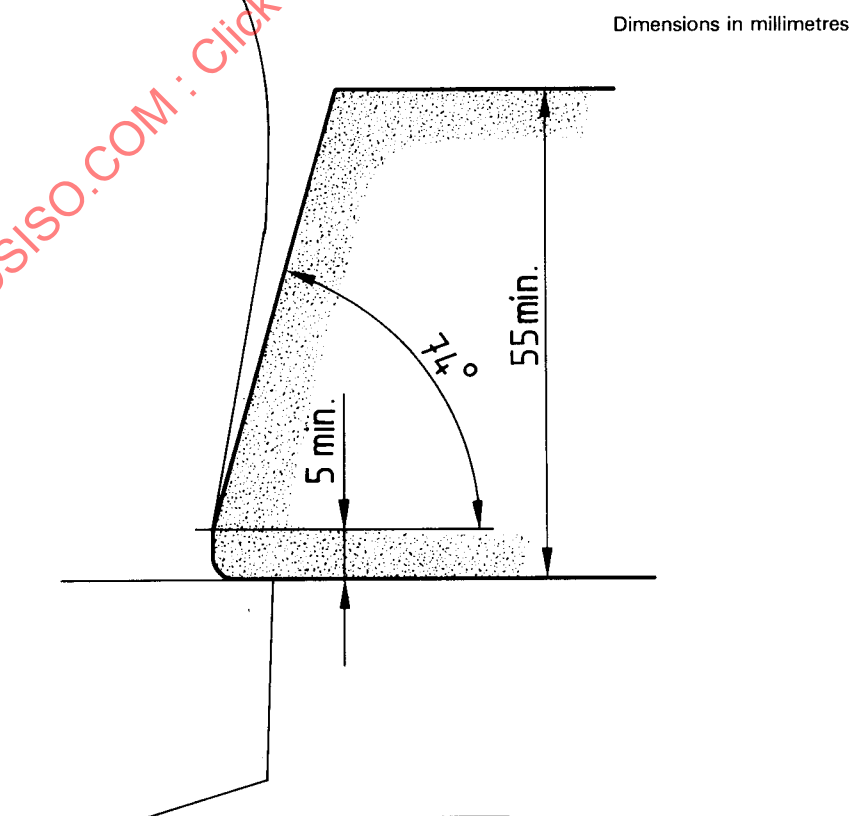
Figure 3 — Free space for the ski binding at the boot heel
