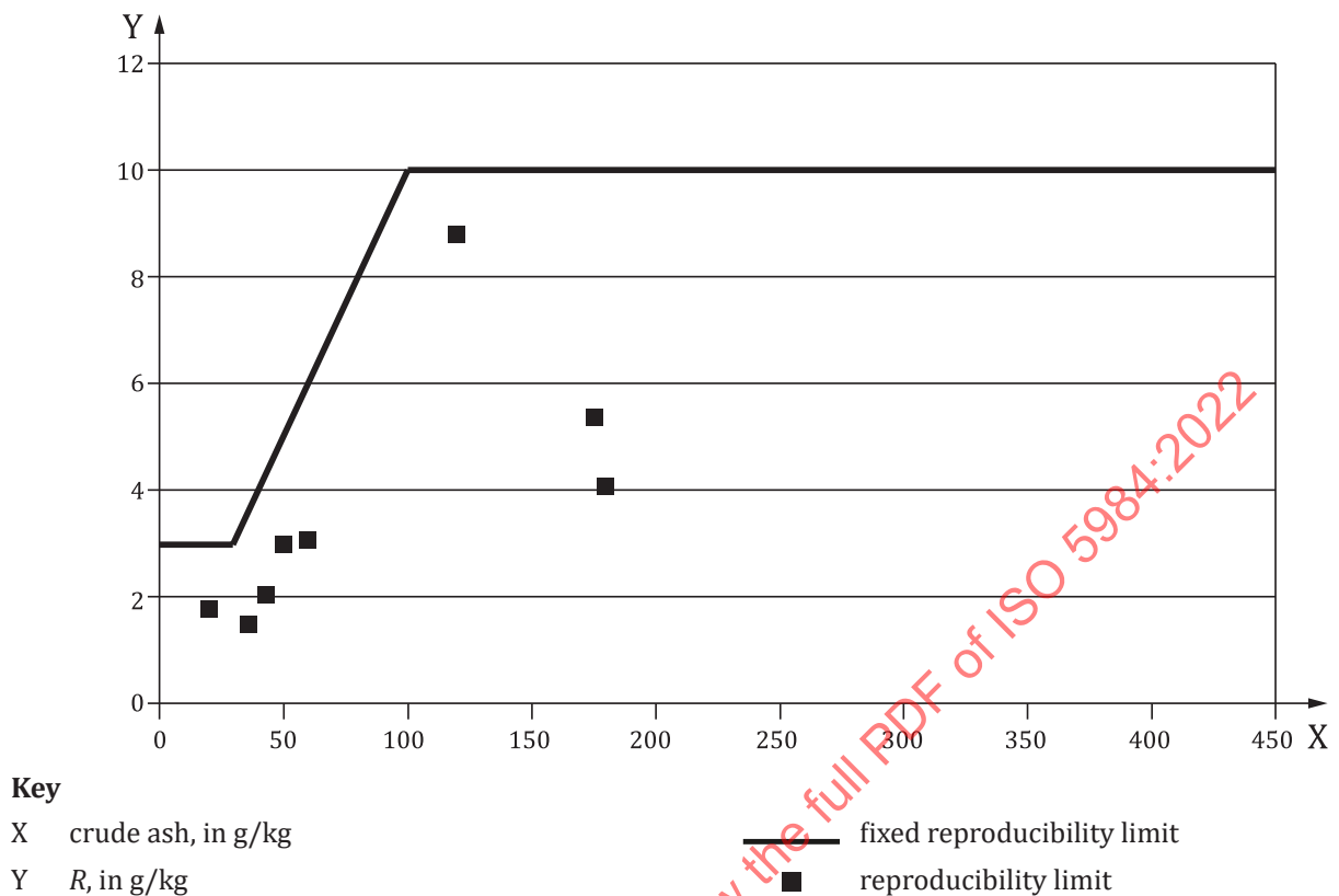
Figure 2 — Graphical representation of reproducibility limit
