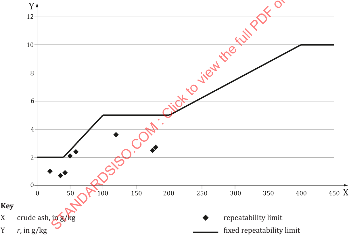
Figure 1 — Graphical representation of repeatability limit
