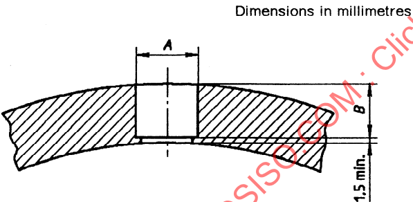
Figure 5 — Socket welding for auxiliary connections
