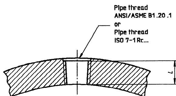
Figure 4 — Thread length for auxiliary connections
